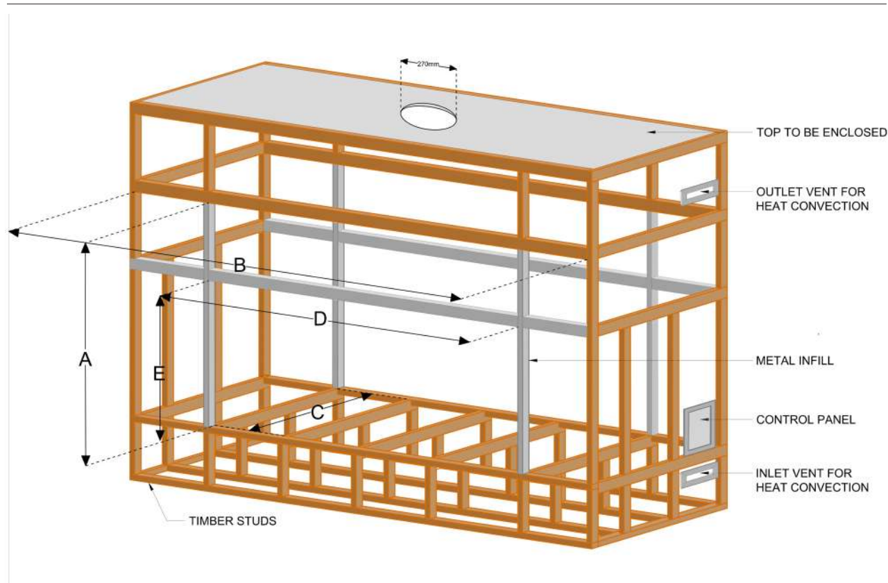
Figure 1.8 (Timber framing)
