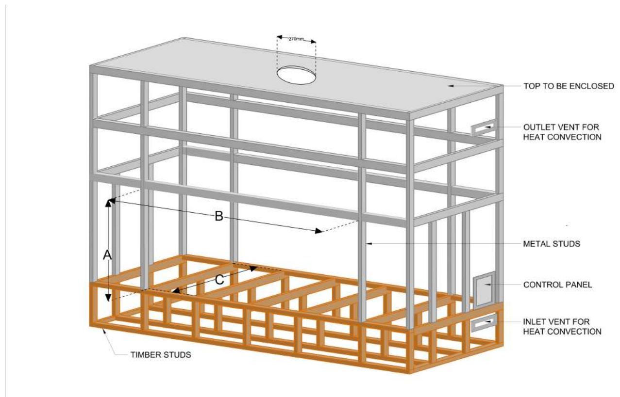
Figure 1.9 (Metal framing)
